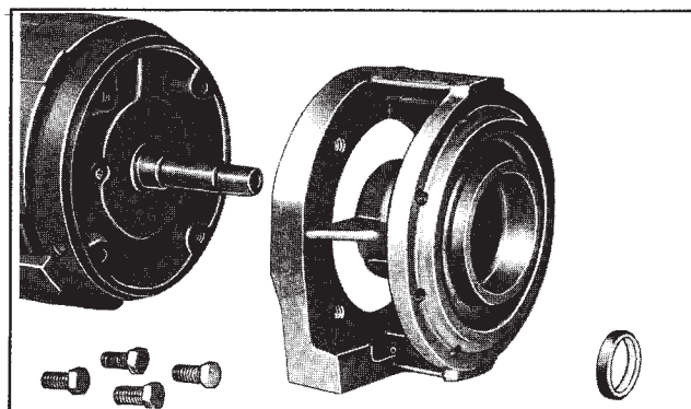
E. Bracket, seal flexible cup and stationary seat removed.
